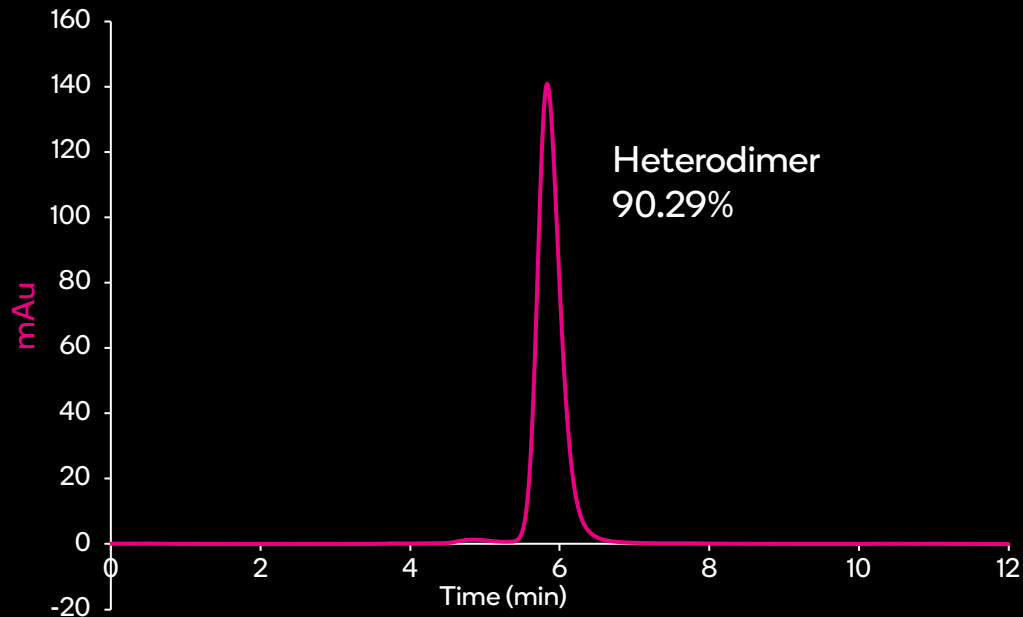
SEC HPLC
